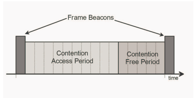
Fig. 1. Superframe structure in 802.15.4
