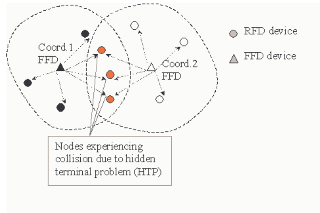
Fig. 3. An example of hidden terminal problem in 802.15.4 due to concurrent transmission of nodes, which belongs to different clusters, that are too far apart to sense each other transmission
