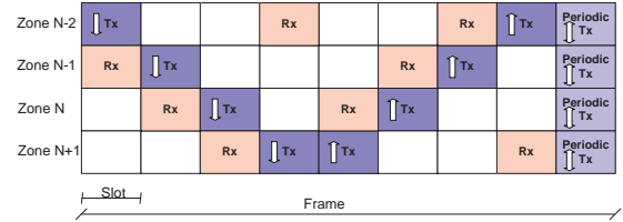
Fig. 6. The table of scheduling with periodic local broadcast
