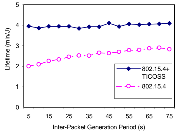
Fig. 9. A comparison of the network lifetime between 802.15.4 with and without TICOSS
