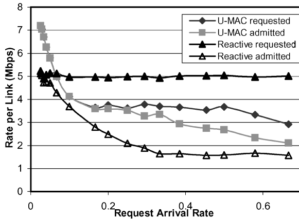
Fig. 13. Rate per link versus request arrival rate.
