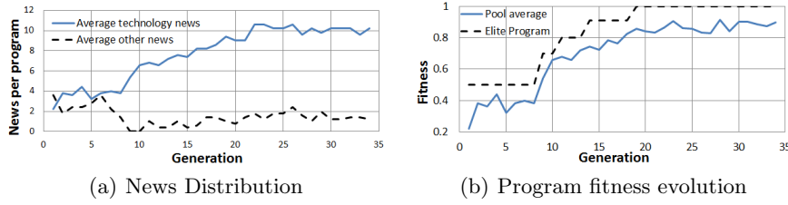
Fig. 4. News Distribution and Program fitness evolution
